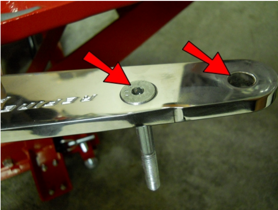
Insert a 3/8-16x3.5" Flat Head Bolt into the countersunk hole and a 1/2-20x2.75" Hex Head Bolt into the other hole on the back side of the FC14-R.
