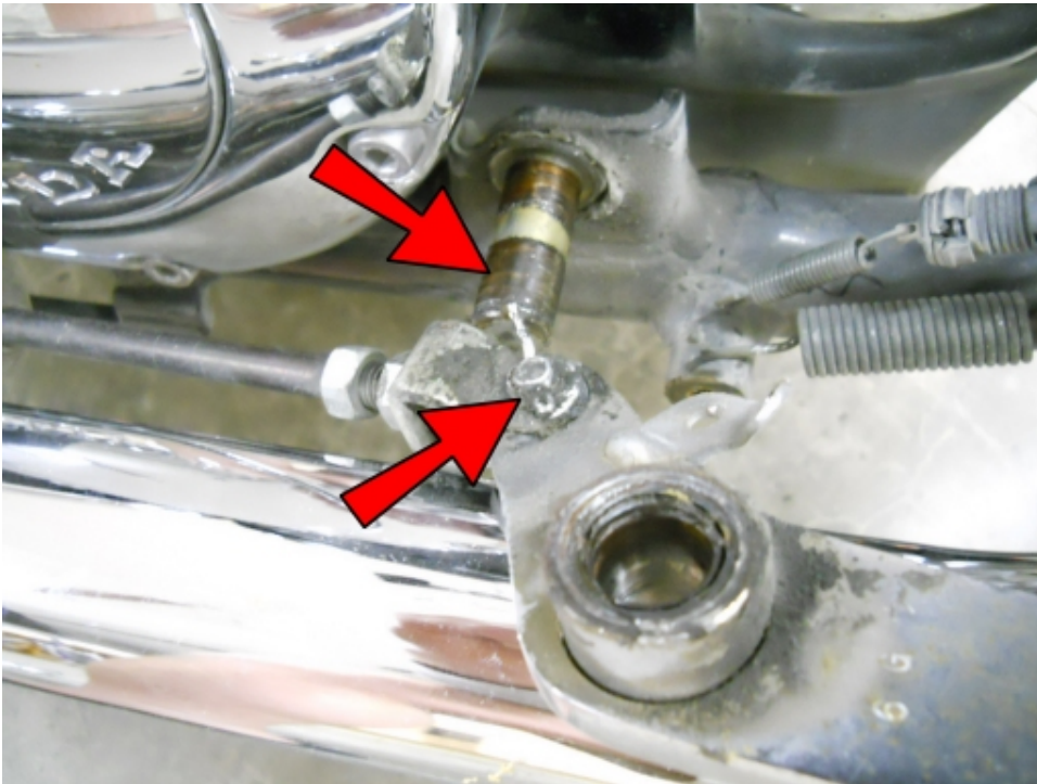
Remove the brake pedal from the shaft. Note: You may have to loosen the exhaust a little. Remove the cotter pin and clevis pin to remove the brake pedal from the linkage.
