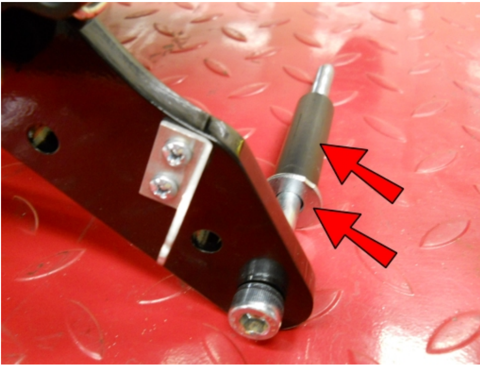
Place a 3/8 Washer and a 2.8" Spacer onto the back side.
