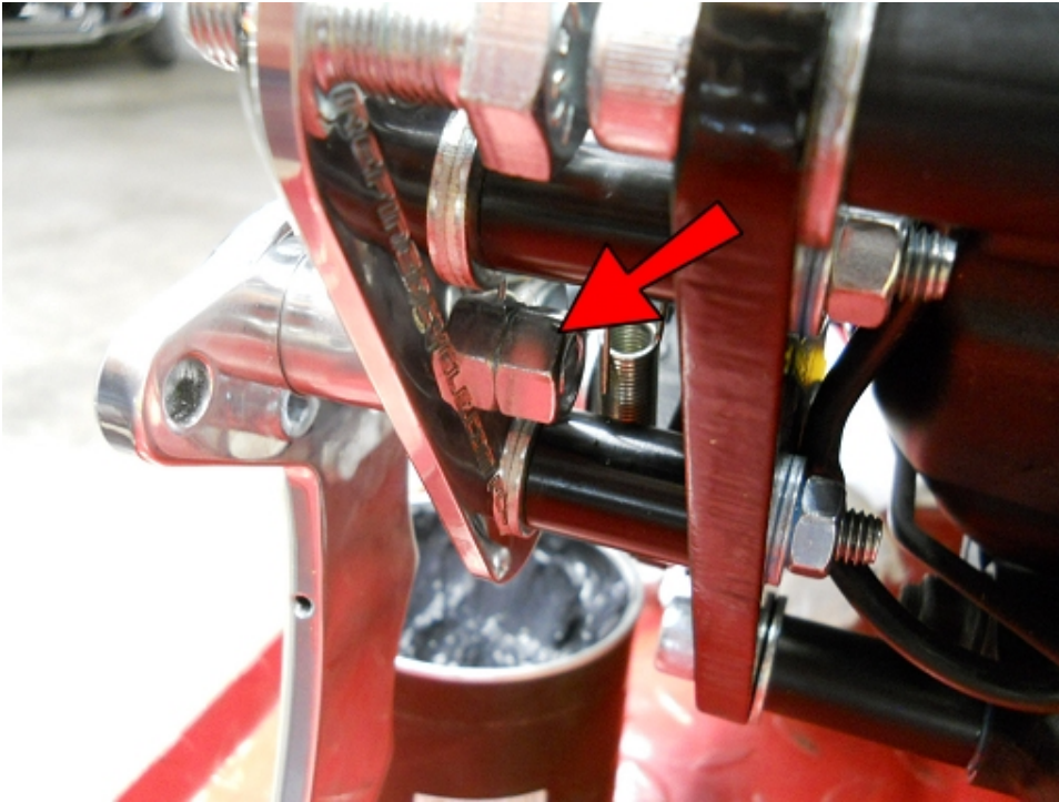
Connect the Brake Pedal to the Right Control Plate and secure with a 3/8 Nut.
