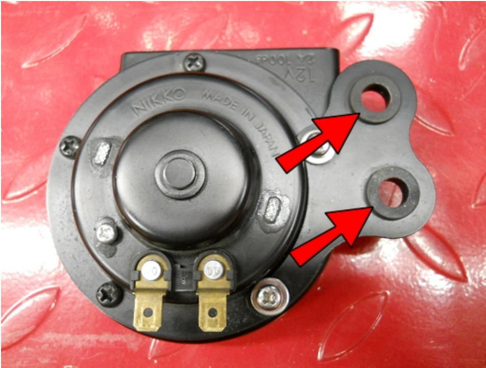
Remove these rubber grommets.
