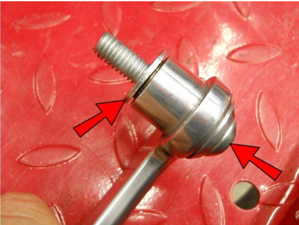
Insert a 3/8-16x2 BHCS into the Shifter Pedal that you previously put the greased sleeves into. Then slide a 5/16 Washer on.
