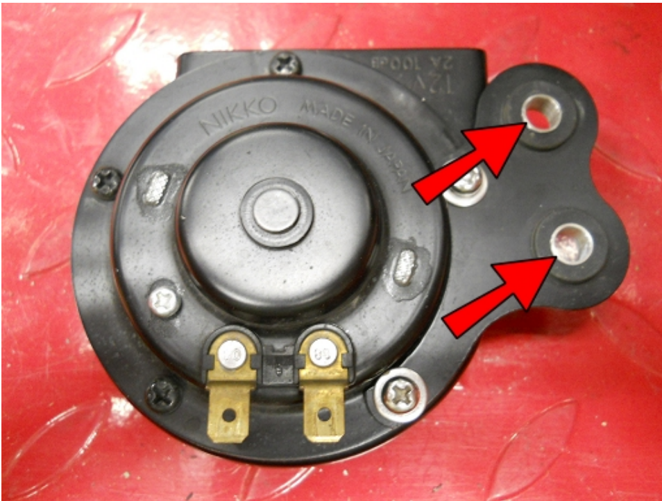
Remove these steel sleeves.
