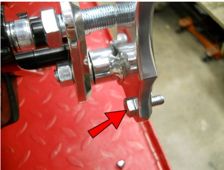
Thread the M6-1.0x18 Bolt into the back side of the Shifter Pedal.
