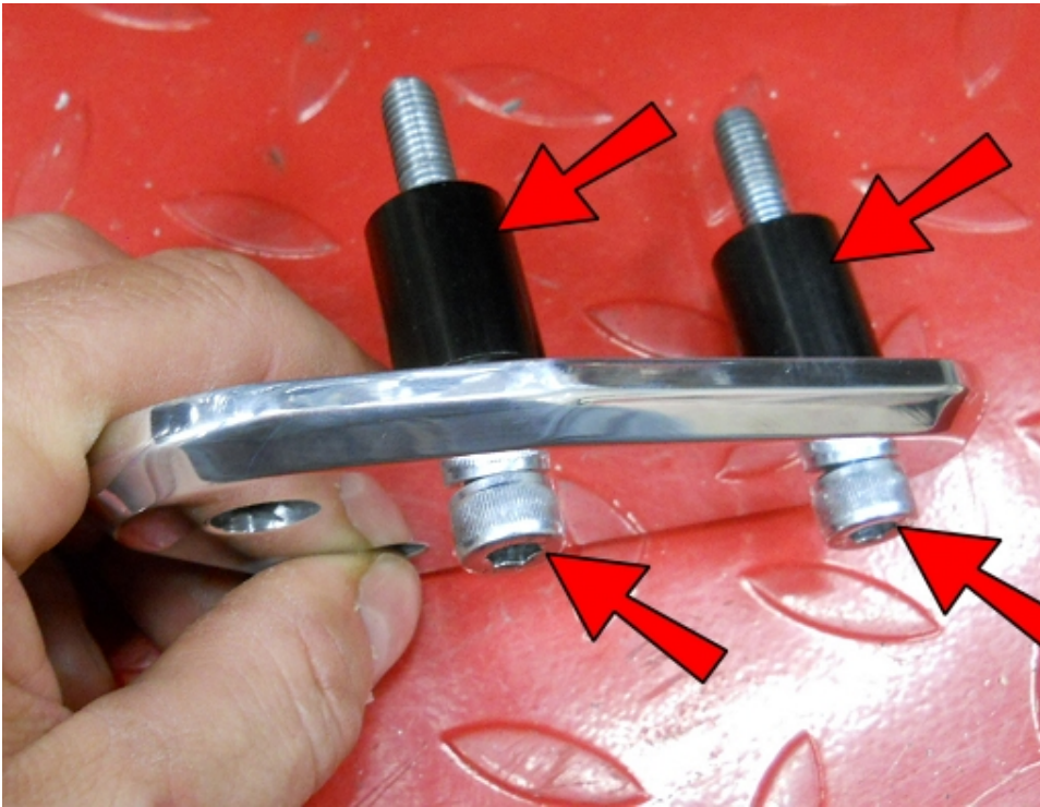
Insert M8-1.25x60 SHCS's into the Left Control Plate then slide 1" Spacers on the back side.
