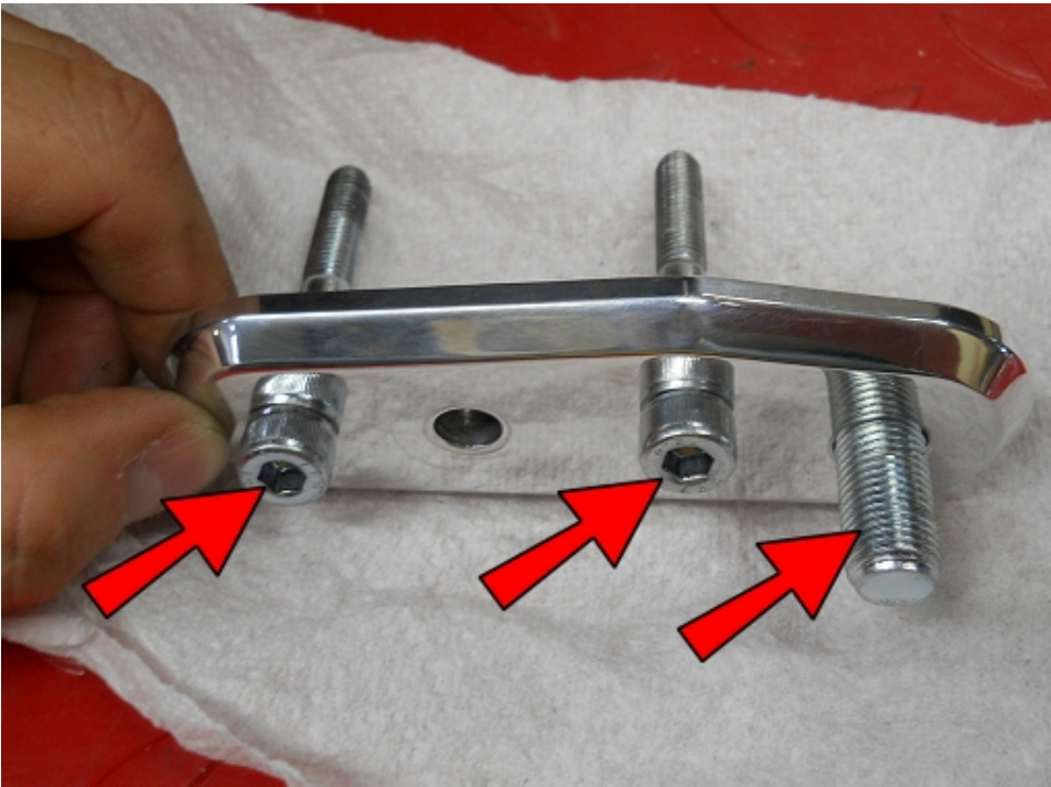
Insert two M8-1.25x60 SHCS's and a foot peg bolt into the Right Control Plate as shown.
