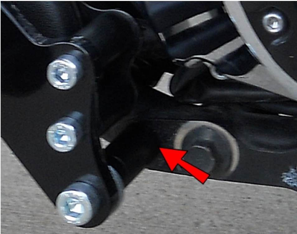
Secure the bolt into the frame, then tighten the M10-1.25x170 SHCS and Nut started previously.
